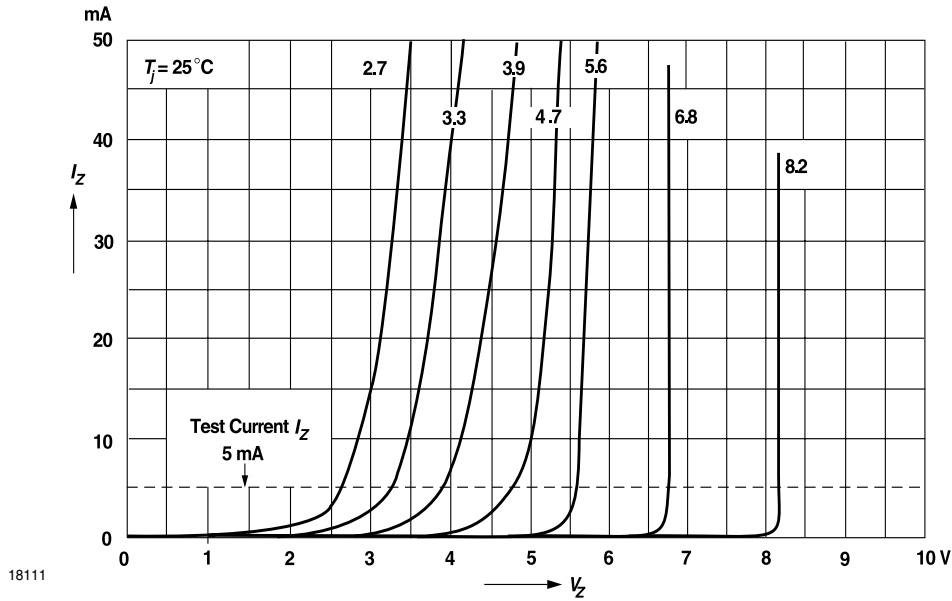
Figure 16. Breakdown Characteristics
