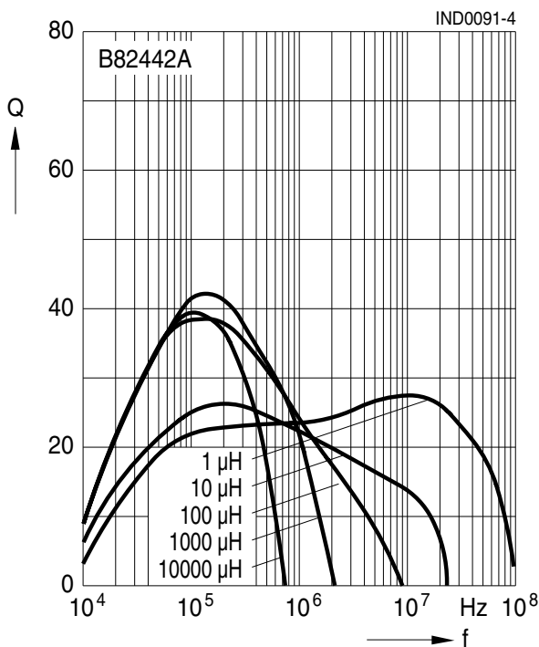
Q factor versus frequency f measured with impedance analyzer Agilent 4191A/4194A, typical values at 20 °C
